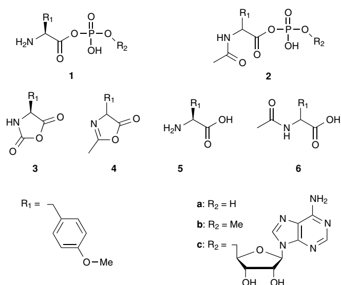
Figure 4 | Structure of the reactants and products related to O -methyltyrosine (H-Tyr(Me)-OH) 5 studied in this work.
