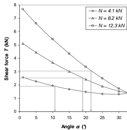
Figure 10. Determination of angle \alpha for different normal loads N ( \alpha = \beta )
