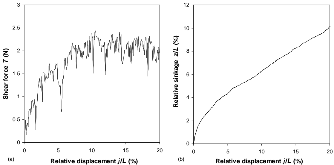
Figure 7. Numerical test (grousers, N = 5 \text{ N} , fast speed), (a) ( j/L, T ) curve, (b) ( j/L, z/L ) curve
