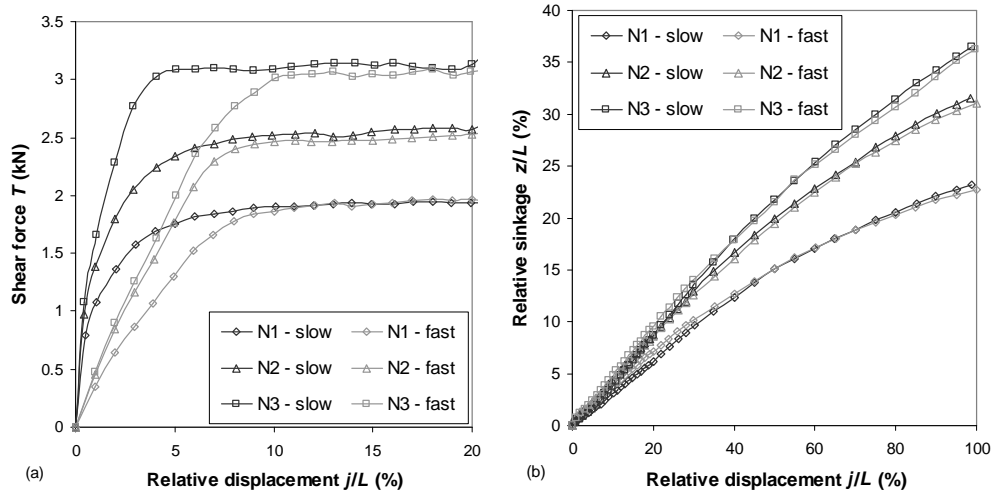
Figure 6. Influence of the translation speed (slow speed = 23 mm.min -1 , fast speed = 14 mm.s -1 ) during shear tests with alveolate plate (normal load N1 = 50 kPa, N2 = 100 kPa, N3 = 150 kPa) on D1 sand (a) mean values ( j/L , T ) curves, (b) mean values ( j/L , z/L ) curves
