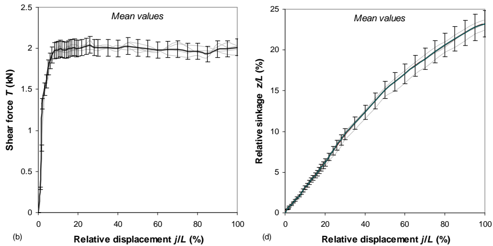
Figure 5. Translation shear test, (alveolate plate, normal stress \sigma = 50 kPa, slow speed = 23 mm.min -1 ) (b) mean values ( j/L , T ) curve ( \Delta = 5\% ), (d) mean values ( j/L , z/L ) curve ( \Delta = 7\% )
