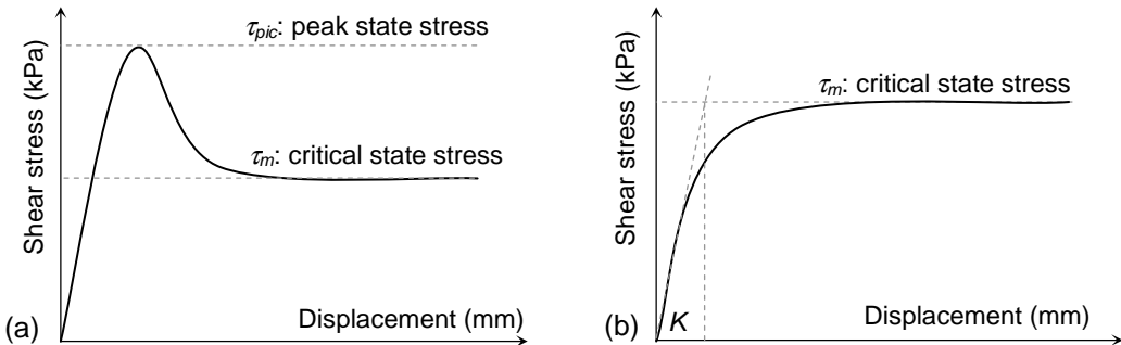
Figure 2. Shear-displacement curves (a) with a peak state, (b) without a peak state
