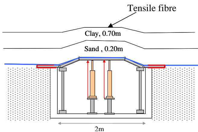
Figure 4: Burst test
