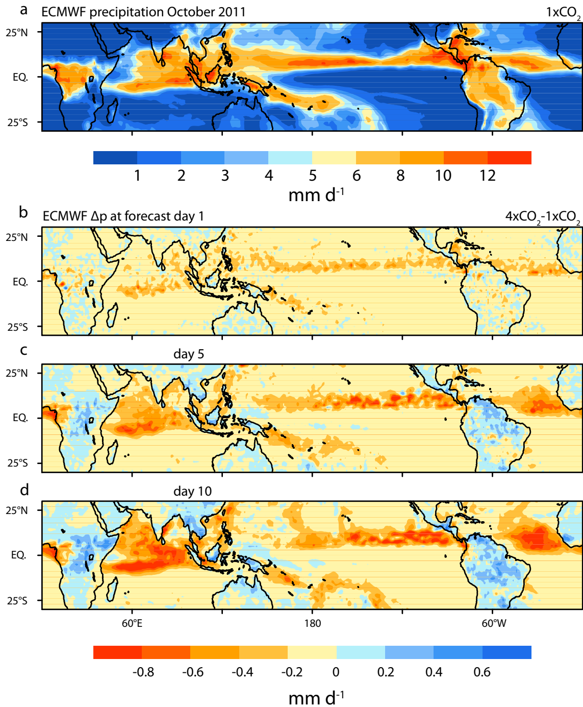
Figure S7: Direct effect of \text{CO}_2 simulated by an operational Numerical Weather Prediction model. (a) Monthly-mean tropical precipitation derived from ECMWF-IFS forecasts for October 2011 using present-day \text{CO}_2 concentration. (b-d) Change in the October 2011 monthly-mean precipitation associated with a quadrupling of the \text{CO}_2 concentration in the atmosphere, shown for different forecast times (1 day, 5 days and 10 days).
