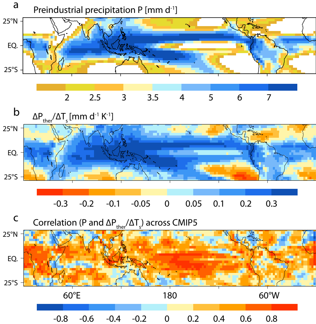
Figure S4: Correlation between precipitation climatology and the thermodynamic component of precipitation changes (a) Multi-model mean pattern of annual precipitation (in \text{mm d}^{-1} ) derived from 16 CMIP5 OAGCMs in the pre-industrial climate (piControl). (b) Multi-model mean pattern of the thermodynamic component of precipitation changes normalised by the local surface warming ( \Delta P_{\text{ther}}/\Delta T_s , expressed in \text{mm d}^{-1} \text{K}^{-1} ) inferred from the same models in abrupt4xCO2 experiments. (c) Correlation (computed across 16 CMIP5 models) between the precipitation climatology and the thermodynamic component predicted by individual models.
