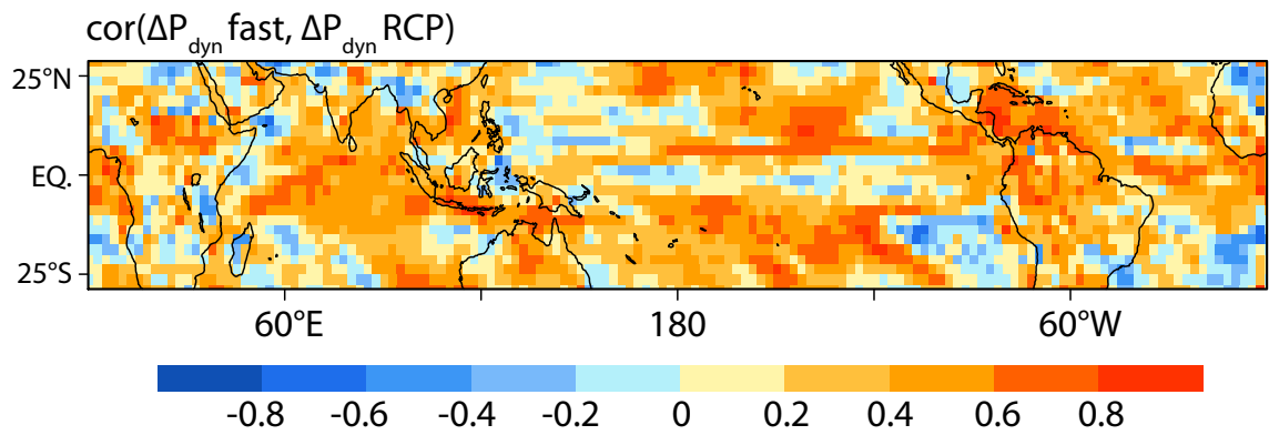
Figure S6: Inter-model correlation between fast and long-term dynamic components of precipitation changes. The figure shows the linear correlation coefficient (computed across 14 CMIP5 models) between the fast dynamic response of precipitation to increased \text{CO}_2 ( \Delta P_{\text{dyn fast}} , inferred from the first year of abrupt4x \text{CO}_2 experiments) and the long-term dynamic response of precipitation ( \Delta P_{\text{dyn RCP}} , estimated from RCP8.5 experiments at the end of the 21 st century).
