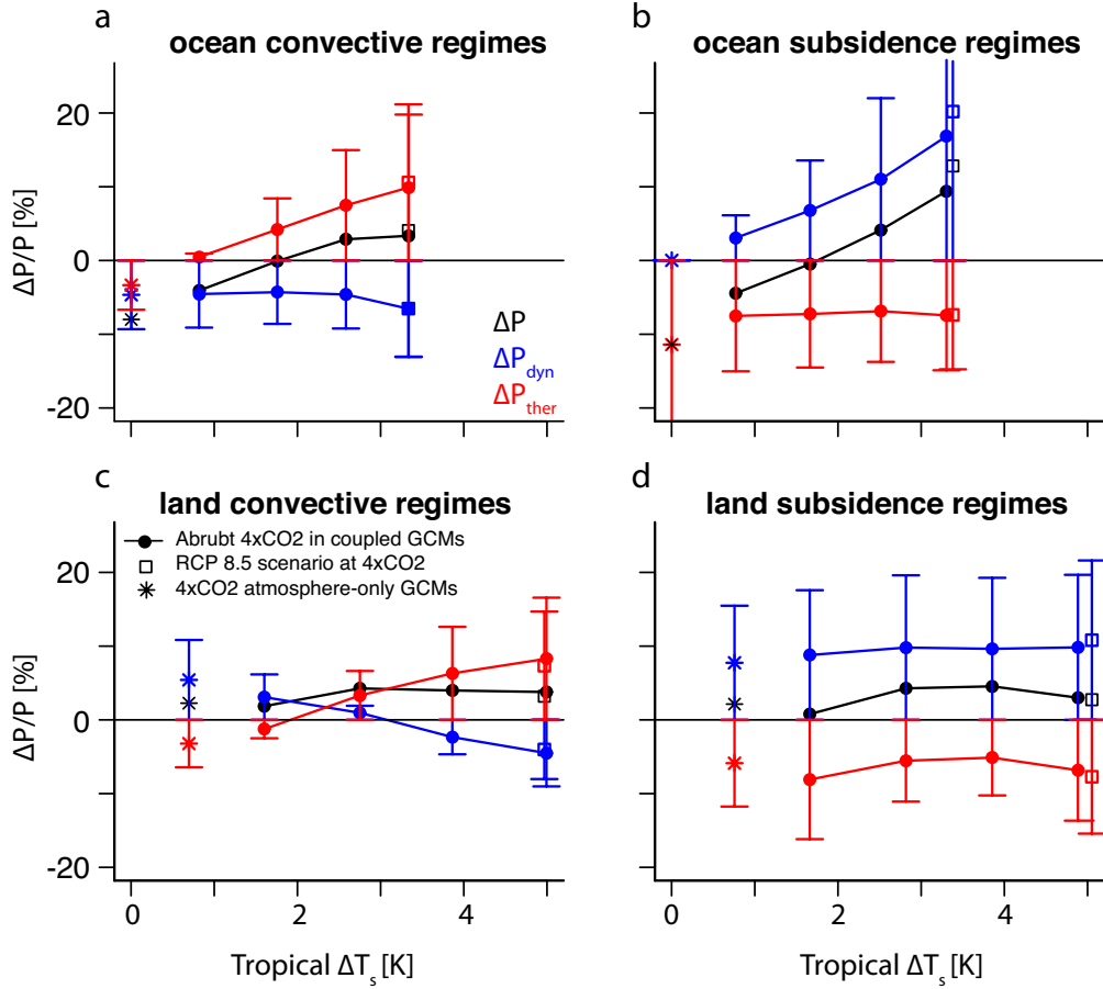
Figure S1: Evolution of precipitation as a function of \text{CO}_2 and surface warming. The different panels show the evolution, as a function of tropical surface warming, of the annual-mean precipitation ( \Delta P = \Delta P_{\text{dyn}} + \Delta P_{\text{ther}} ) predicted by CMIP5 models in pre-industrial regimes of large-scale ascent ( \bar{\omega} < 0 , also named "convective" regimes, left panels) or large-scale subsidence ( \bar{\omega} > 0 , right panels). Results are reported for several CMIP5 experiments : for abrupt4xCO2 coupled ocean-atmosphere experiments (first 30 years of simulation after \text{CO}_2 quadrupling), for non-mitigated climate change scenario experiments at the end of the century (RCP8.5, around 2090), and for equilibrium atmosphere-only experiments in which the \text{CO}_2 concentration is quadrupled but sea surface temperature are kept unchanged (sstClim4xCO2, averaged over 30-years). Fractional changes relative to pre-industrial values are expressed in %. Vertical bars show \pm one inter-model standard deviation of individual model results around the multi-model mean.
