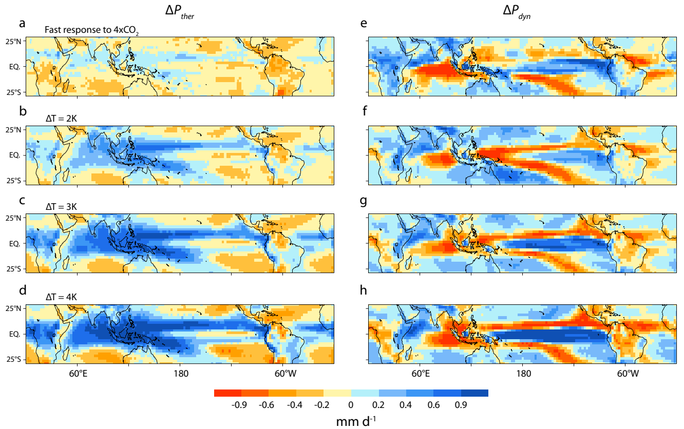
Figure 2: Interpretation of the multi-model mean regional pattern of tropical precipitation changes induced by a \text{CO}_2 increase. Decomposition into thermodynamic (a-d, \Delta P_{\text{ther}} ) and dynamic (e-h, \Delta P_{\text{dyn}} ) components of the annual-mean precipitation change predicted by CMIP5 coupled ocean-atmosphere models at different stages of an experiment in which \text{CO}_2 is abruptly quadrupled: (a, e) for the first year after \text{CO}_2 quadrupling, and for a tropical surface warming of (b, f) 2 K, (c, g) 3 K, (d, h) 4 K. Note the resemblance between the patterns simulated for a 4 K surface warming in this experiment and those projected by the end of the 21 st century in the RCP 8.5 scenario (Figure 1c-d).
