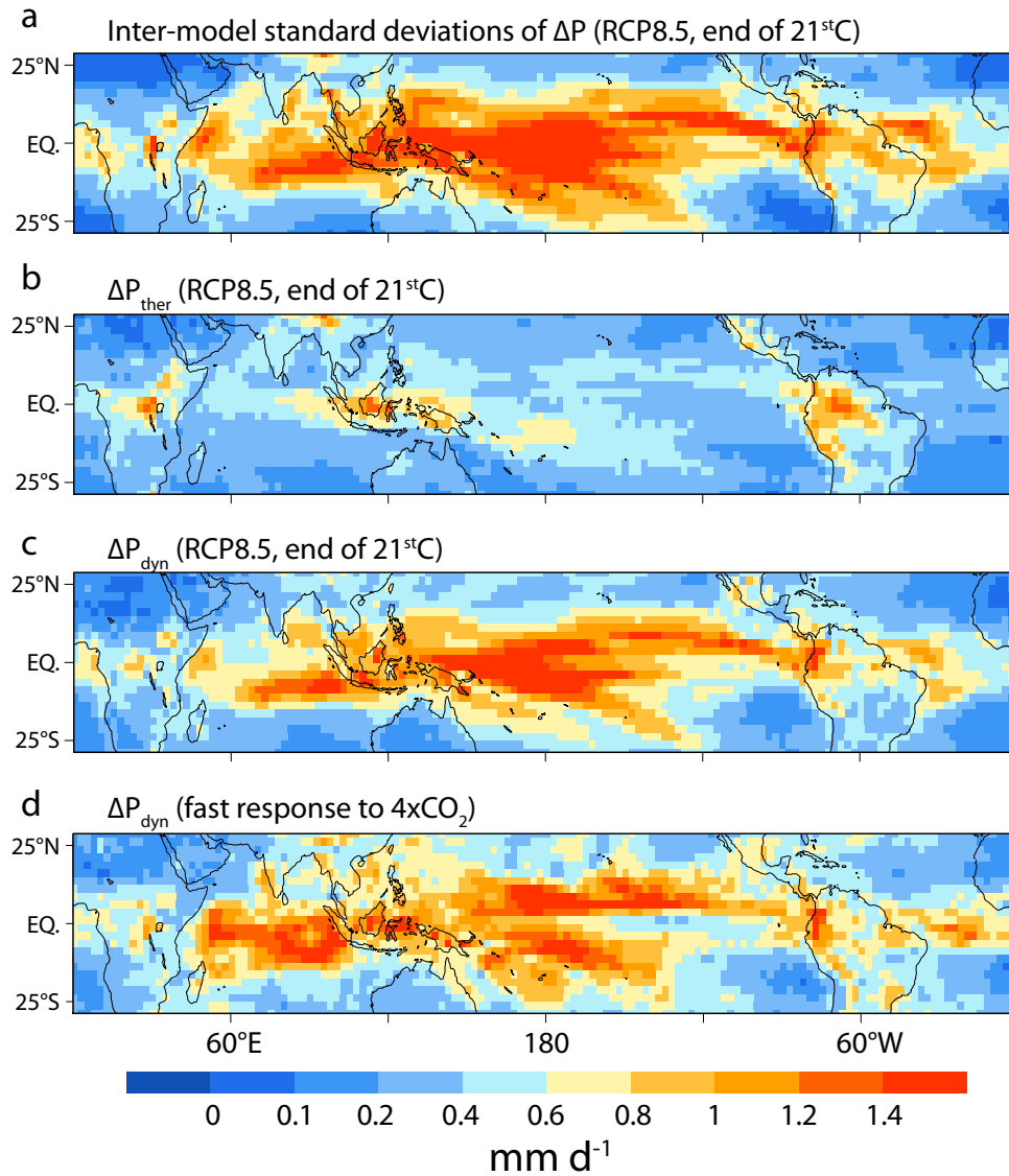
Figure S8: Inter-model spread of regional precipitation projections in the tropics. (a) Spread (inter-model standard deviation, in \text{mm d}^{-1} ) of precipitation changes projected by 14 CMIP5 OAGCMs in the RCP8.5 scenario at the end of the 21 st century. (b) and (c) Spread of the thermodynamic and dynamic components of precipitation changes in the same models and the same scenario. (d) Spread of the fast dynamic component of precipitation changes inferred from the first simulated year of abrupt4xCO 2 experiments. The tropical-mean standard deviations of the different panels from top to bottom are: 0.69, 0.35, 0.58 and 0.63 \text{mm d}^{-1} .
