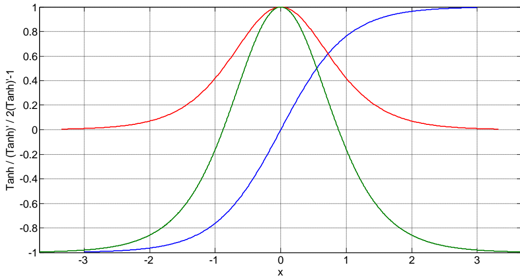
Fig. 1: In blue the tanh function and in red its derivative ( = 1 - \tanh^2 ). The green curve represents the scaled form of (\tanh)'
