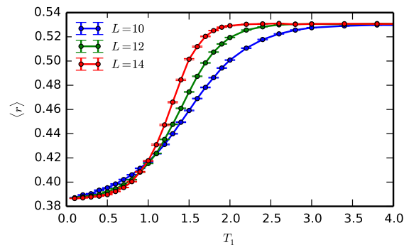
FIG. 1. Disorder-averaged level statistics parameter \langle r \rangle as a function of the “kick” strength T_1 . At small values of T_1 , \langle r \rangle \approx 0.386 , indicating Poisson statistics of quasi-energy levels (no level repulsion). At larger T_1 the system undergoes a transition into a delocalized phase with \langle r \rangle \approx 0.53 , consistent with COE [25]. Data is for system sizes L = 10, 12, 14 , and averaging is performed over 1000 disorder realizations.
