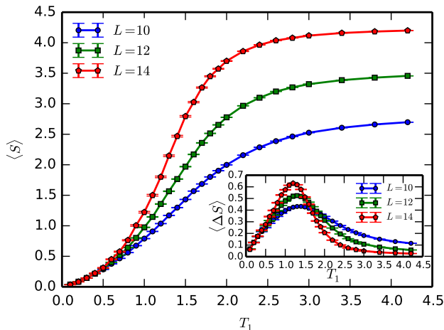
FIG. 2. Averaged entanglement entropy \langle S \rangle and its fluctuations \Delta S (inset) as a function of T_1 . The scaling of entropy and its fluctuations with system size L are consistent with the existence of an MBL and a delocalized phase for small and large T_1 , respectively.
