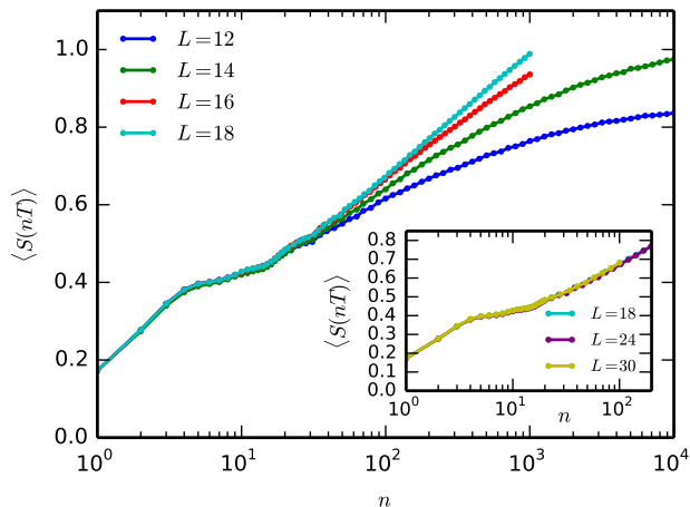
FIG. 4. Disorder-averaged entanglement entropy following a quantum quench, for the Néel initial state. Data for system sizes L = 12, 14 was obtained by ED, for L = 16, 18 using Krylov subspace projection, and L = 24, 30 using TEBD. Averaging performed over 6000 disorder realizations.
