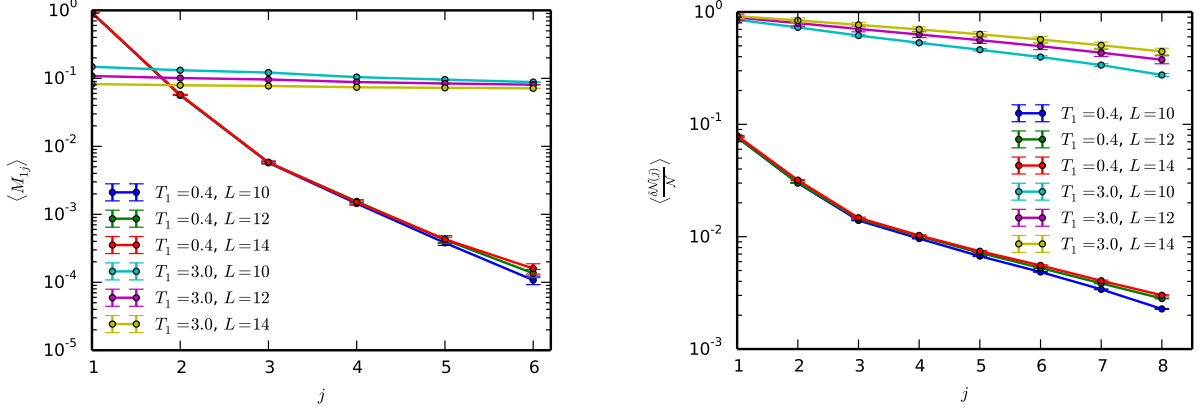
FIG. 6. Local integrals of motion in the MBL and delocalized phase. (Left) Median magnetization M_{1j} as a function of distance |1 - j| . (Right) Median difference between the total norm \mathcal{N} , and partial norm \delta\mathcal{N}(j) , divided by \mathcal{N} . The exponential decay of this quantity with distance |j - 1| demonstrates that in the MBL phase ( T_1 = 0.4 ) operator \bar{\sigma}_1^z is a quasi-local integral of motion. In the delocalized phase ( T_1 = 3 ), this operator becomes non-local.
