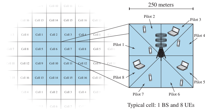
Fig. 1. The simulation scenario considers 16 square cells with wrap-around to avoid edge effects. Each cell is 250 m \times 250 m and consists of 8 UEs uniformly distributed in different parts of the cell.
