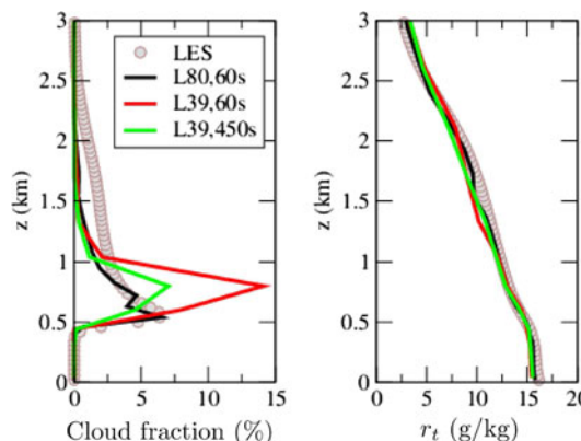
Fig. 5 Effect on the LMDZ5B single-column simulations of the Rico case of changing the vertical grid or time step. We show the mean cloudiness (left) and specific humidity (g/kg, right) profiles averaged between hour 6 and 12 of the simulation. The single-column integration shown in Figs. 1 and 8 are run with the L80 vertical grid and a time step of 60 s. They correspond to the black curve here. The L39 grid is that of the 3D model. The green curve corresponds to the L39 vertical discretization and 450 s time step of the 3D climate simulations
