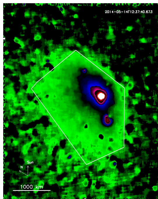
Fig. 7. Comet 67P/Churyumov-Gerasimenko observed with the OSIRIS NAC orange on May 14 at 12:37:41. A background star image has been subtracted. The directions to the Sun and celestial north are marked. The white polygon indicates the image area used to compute the total mass lost.
