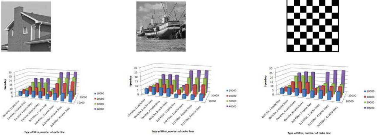
Figure 2. Exploration of cache-line structure with 1x8 block size
