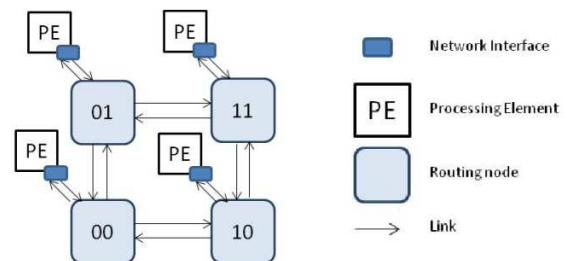
Fig 1. Basic elements for the NoC structure.
