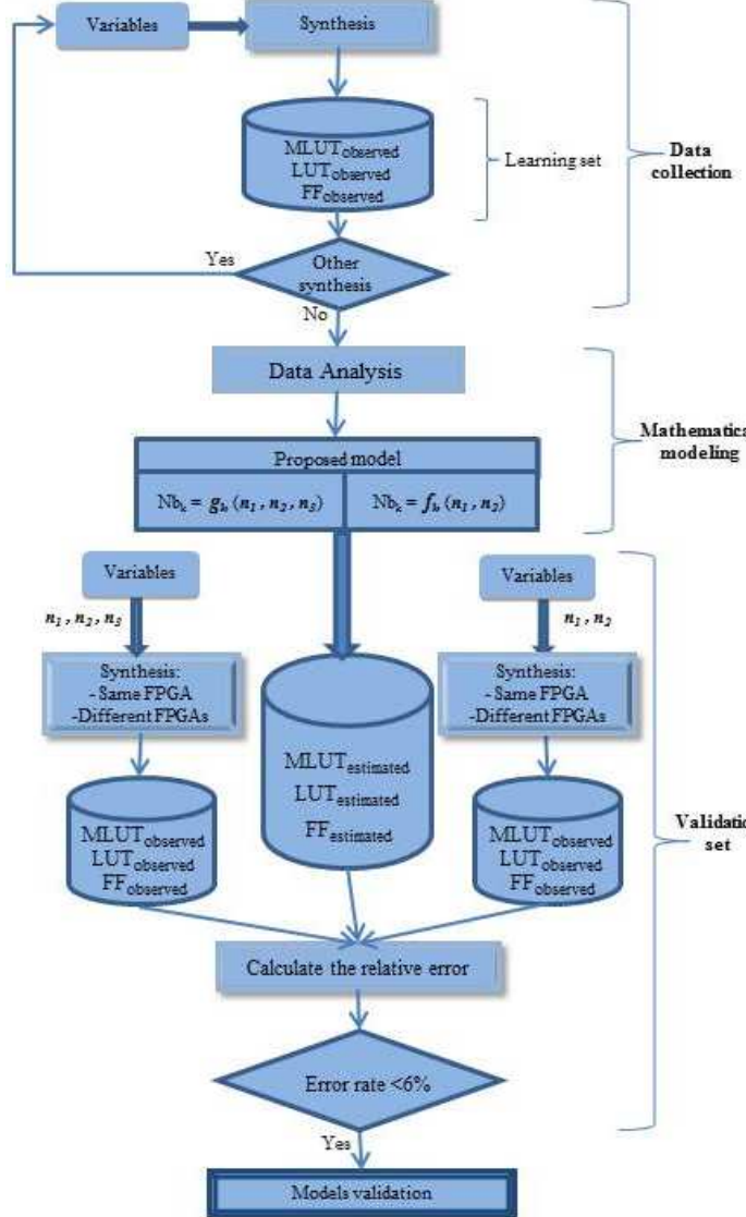
Fig 2. Methodological framework
