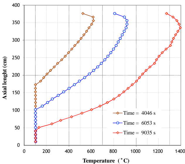
Figure 4: Axial temperatures of fuel rods in the central part of an isolated assembly (decay heat = 58kW) during dewatering
