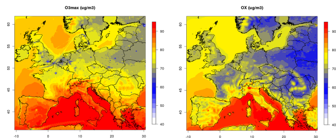
Figure 28. In a continental chemistry transport simulation with the CHIMERE model at a resolution of 8 km, major urban centres in northern and central Europe highlight the \text{NO}_x titration process (left: summertime average of daily maximum ozone), while the total oxidant level (right: \text{O}_3 as \text{NO}_2 + \text{O}_3 , annual mean) is high in most European cities (adapted from Terrenoire et al., 2015).
