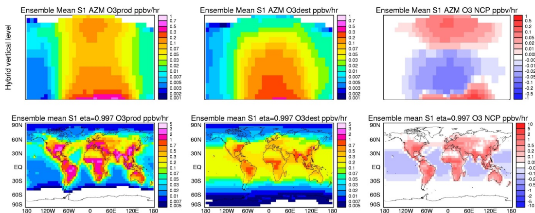
Figure 2. Multi-model mean (20 models) year 2000 ozone budgets (units: \text{ppb h}^{-1} ). Top row: annual zonal mean (AZM) chemical production, chemical destruction and net chemical production. Vertical scale is from surface to approximately 100 hPa. Bottom row: maps of same quantities in the surface model layer (Stevenson et al., 2006).
