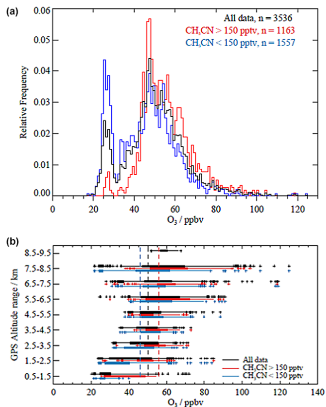
Figure 31. (a) Frequency distribution for ozone over the BORTAS (Palmer et al., 2013) flights, the black line are the measured mixing ratios, where the red line shows the distribution of measurements identified as biomass burning plumes using a threshold of \text{CH}_3\text{CN} mixing ratios greater than 150 pptv, and the blue line shows measurements made in air masses with \text{CH}_3\text{CN} mixing ratios less than 150 pptv. (b) The same data plotted as box-and-whisker plots (solid boxes show the range of the 25th to 75th percentiles and whiskers show the range of the 5th to 95th percentiles, with outliers shown as plus symbols) (GPS) altitude profile (Parrington et al., 2013).
