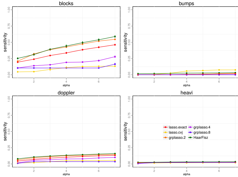
(b) Sensitivity of selection.
