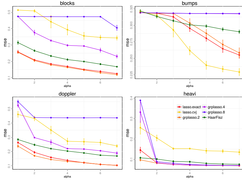
(a) Mean Square error of reconstruction.
