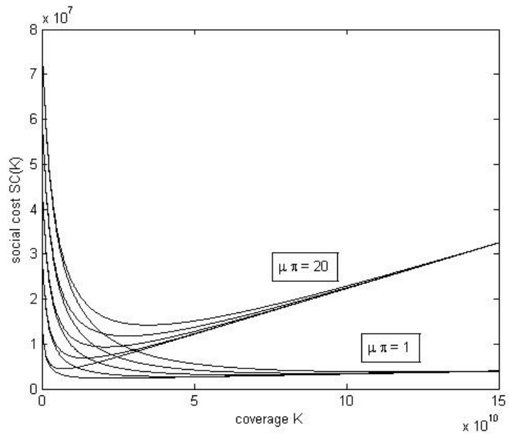
Figure 7: \mu = 1, 20 \quad \pi = 10^{-5}
