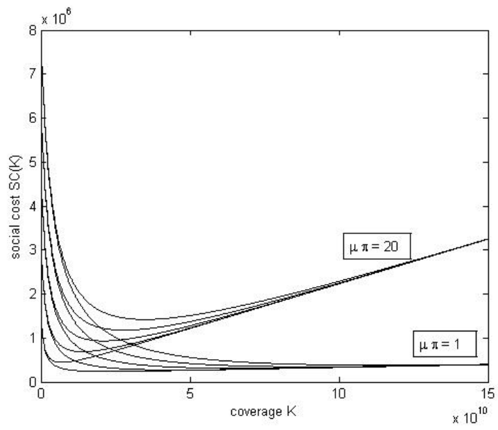
Figure 8: \mu = 1, 20 \quad \pi = 10^{-6}
