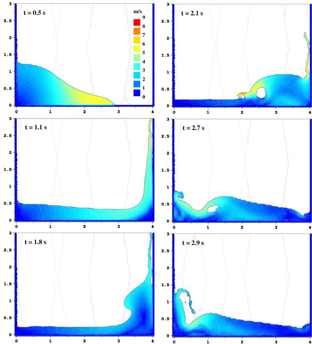
Figure 8. Collapse of a water column in a tank simulated with the present SPH k-\epsilon model. Velocity magnitude distribution at various stages (the legend applies to all the snapshots). To clarify the visualisation, the fields were interpolated on a spatial grid (not involved in the SPH computation).
