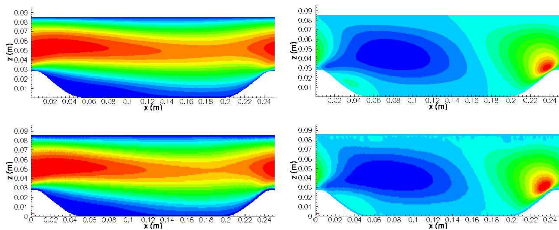
Figure 3. 2D laminar periodic hill flow simulated with a finite volume method (top) and with present SPH model (bottom). Axial (left) and vertical (right) velocities. The SPH velocity fields were time-averaged to reduce numerical fluctuations.
