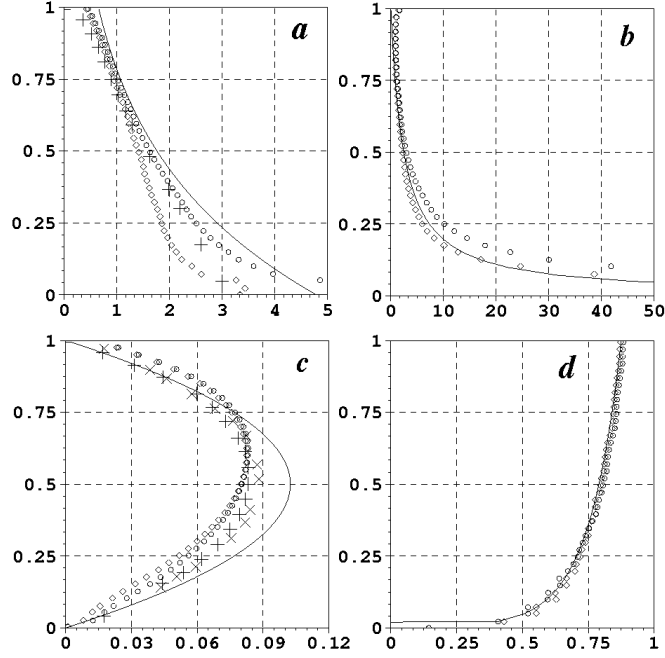
Figure 11. Open-channel turbulent steady flow. Vertical distributions of k / u_*^2 (a), \varepsilon H / u_*^3 (b), \nu_T / Hu_* (c) and axial velocity in m/s (d) versus non-dimensional distance to the bed. Present SPH method with \circ EARSM and \diamond linear k - \varepsilon model; — semi-empirical [20]; \times experimental [20]; + finite elements k - \varepsilon [21].
