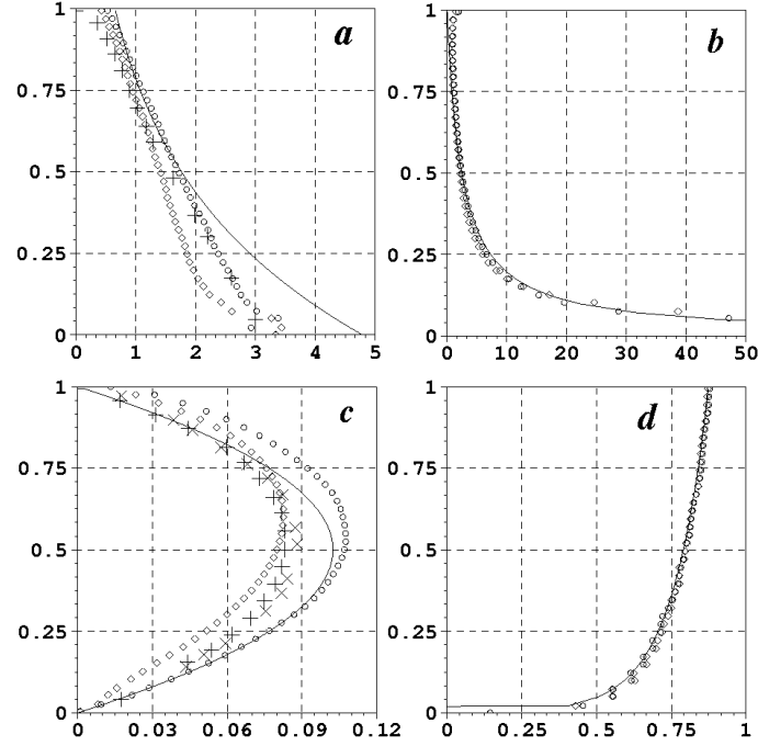
Figure 6. Open-channel turbulent steady flow. Distributions of k/u_*^2 ( a ), \varepsilon H/u_*^3 ( b ), v_T/Hu_* ( c ) and axial velocity in m/s ( d ) versus non-dimensional distance to the bed z/H (on vertical axis). Present SPH method with \circ k-L_m model and \diamond k-\varepsilon model; — semi-empirical [20]; \times experimental [20]; + finite elements k-\varepsilon [21].
