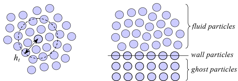
Figure 2. Left: particle interactions are commonly restricted to a finite neighbourhood bounded by a disc
