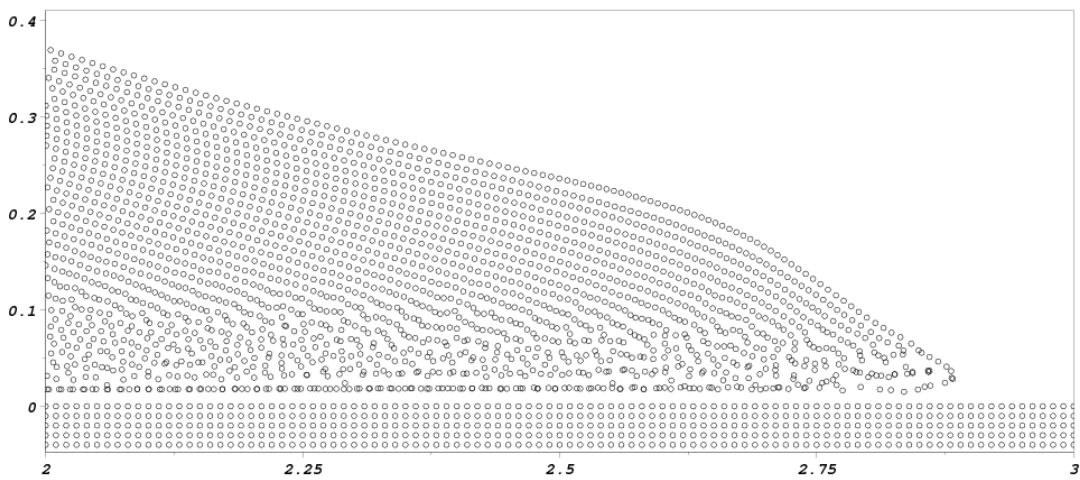
Figure 9. Collapse of a water column in a tank simulated with the present SPH k-\epsilon model. Zoom on the particle positions near the wave front at t = 0.5 s (axis are labelled in meters).
