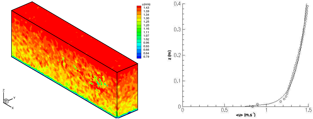
Figure 13. 3D turbulent open-channel flow simulated with the present SPH LES model. Left: 3D turbulent velocities. Right: vertical profile of averaged axial velocity; \circ present SPH method with LES model; — smooth bed log-law.
