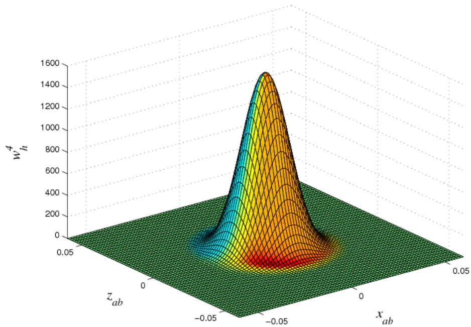
Figure 1. View of the 4 th order spline kernel in two dimensions.
