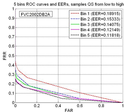
Figure 5: Monotonic increasing matching performance validation of FVC2002DB2A for QMF, calculated by dividing quality values into 5 isometric bins.
