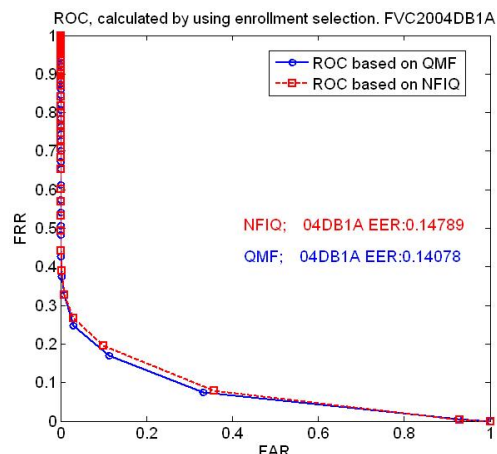
Figure 2: Enrollment selection result of FVC2004DB1A.
