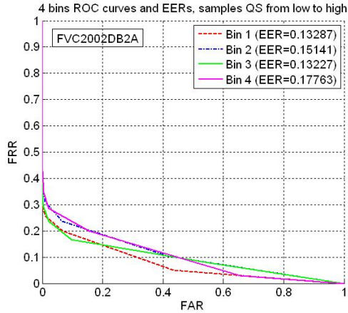
Figure 4: Monotonic increasing matching performance validation of FVC2002DB2A for NFIQ, calculated by dividing quality values into 5 isometric bins (no sample of quality 5 for this database).
