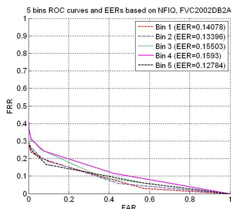
Figure 3: Example of 5-bin evaluation for NFIQ on FVC2002DB2A.
