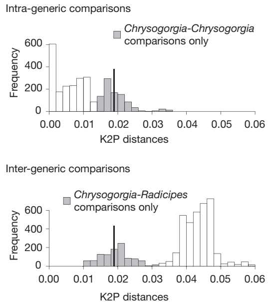
FIG. 9. — Frequency histograms of pairwise genetic distance values (K2P) across 129 chrysogorgiid specimens sequenced at the 5' end of msh1 . Separate histograms are shown for pairwise comparisons made among congeneric individuals (top) and between individuals from different genera (bottom). The vertical black line represents the K2P distance between Pseudochrysogorgia bellona n. gen., n. sp. and its closest relative, Metallogorgia melanotrichos (Wright & Studer, 1889).
