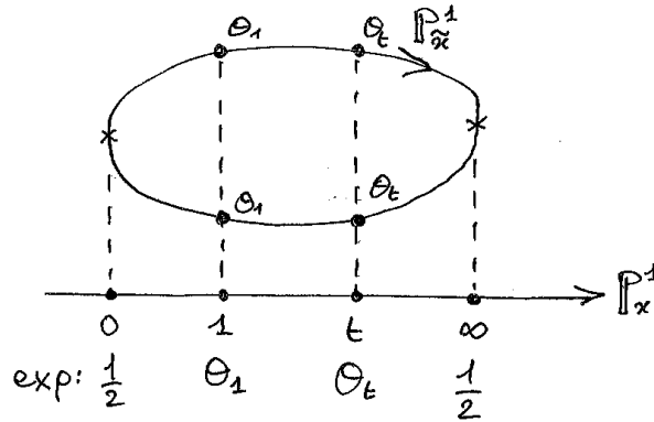
FIGURE 1. Quadratic transformation’s cover
