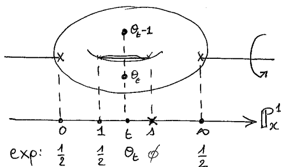
FIGURE 4. Ruled deformations via uncomplete elliptic cover
