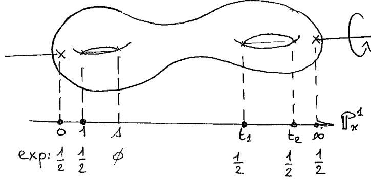
FIGURE 5. Ruled deformations via uncomplete hyperelliptic cover
