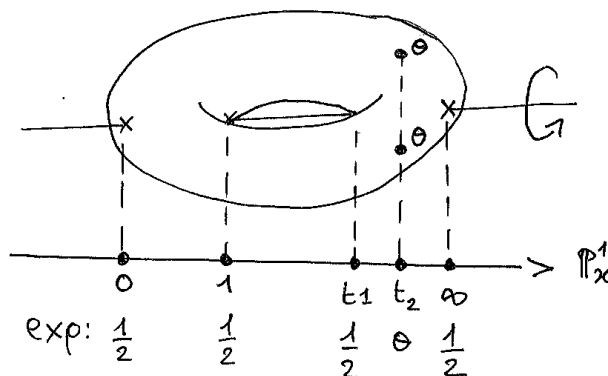
FIGURE 6. The two punctured torus
