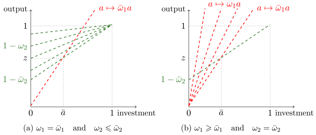
Figure 2: Production functions consistent with z = f(\omega, \bar{a})
