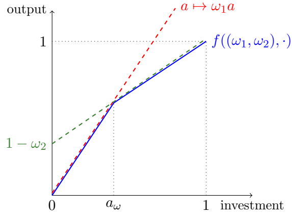
Figure 1: The production function f((\omega_1, \omega_2), \cdot)
