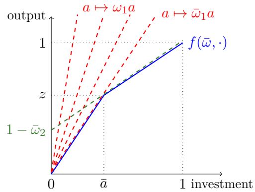
(b) \omega_1 \geq \bar{\omega}_1 and \omega_2 = \bar{\omega}_2
