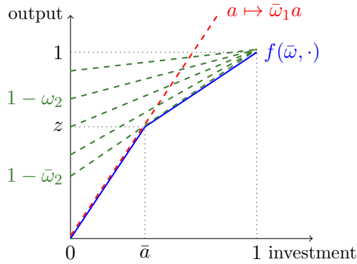
(a) \omega_1 = \bar{\omega}_1 and \omega_2 \leq \bar{\omega}_2
