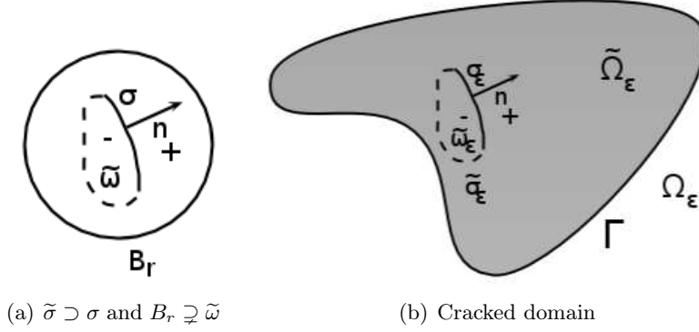
Figure 3: Cracked domain and extension of the crack by a closed curve
