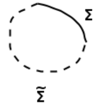
Figure 2: \Sigma and \tilde{\Sigma}
