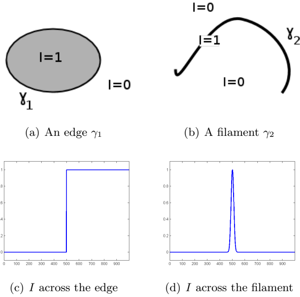
Figure 1: Difference between an edge and a fine structure
