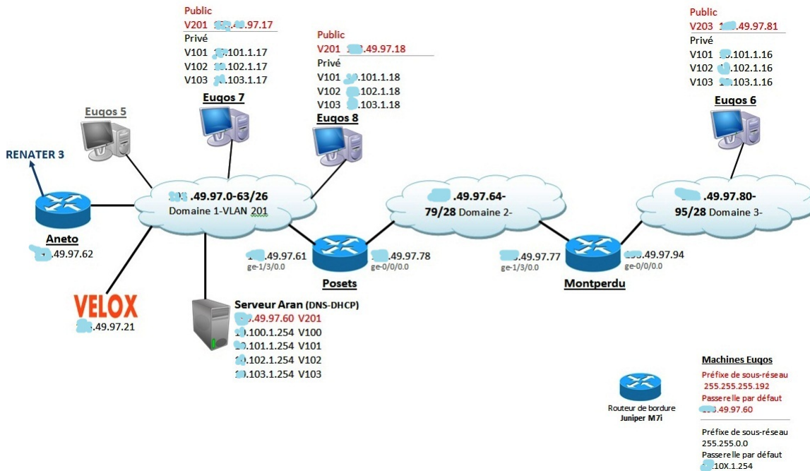
FIGURE 8: Laasnetexp testbed
