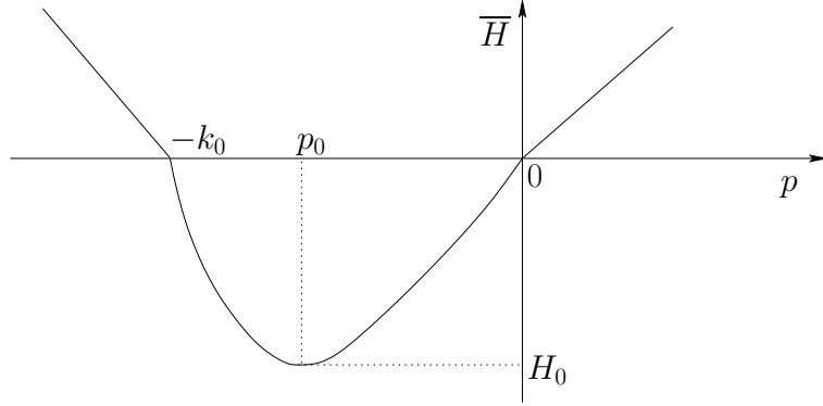
Figure 2: Schematic representation of \bar{H} .
