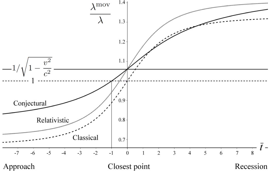
Figure 5. Comparative profiles of Doppler effects predicted for v = c/3 , by the relativistic equation (dotted line), the classical equation (dashed line) and the conjectural Doppler equation calculated here (plain line). Time 0 correspond to wave emission. The switch between the contraction and the dilation occurs at the closest point for the classical formula and before the closest point for the relativistic formula (between -1 and 0, see the text) and for the conjectural function, precisely at \bar{t} = -1 .
