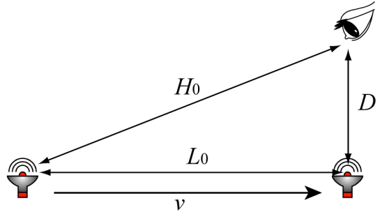
Figure 3. A source moving at constant speed v starts from a distance H_0 from the immobile observer. The shortest distance between the source and the observer is D .
