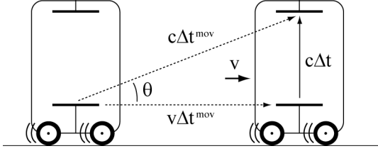
Figure 1. The famous triangular time-space diagram of the moving Einstein's clock. The horizontal scale is artificially stretched relatively to the vertical one for better visualization.
