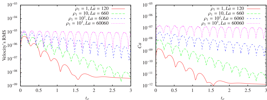
Figure 15: Static column case with variable density: convergence study for the velocity's RMS and Ca number by varying the density inside the column using the CP_\perp method with 2 iterations and order 4 \kappa_{LS} with R/h = 12.8 .
