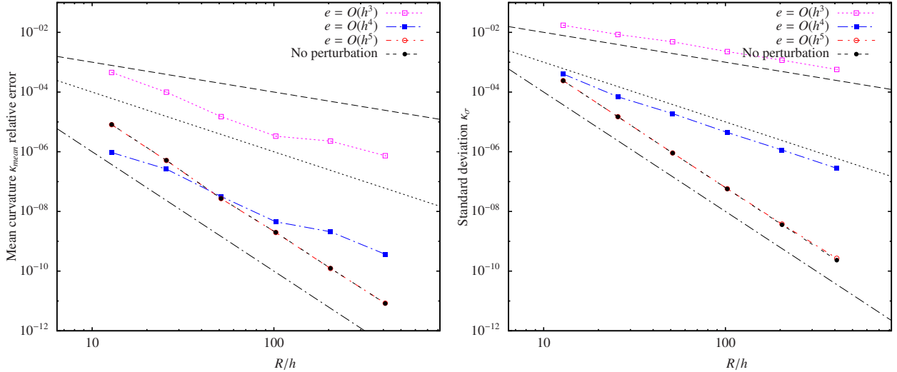
(a) Mean curvature relative error and standard deviation.
