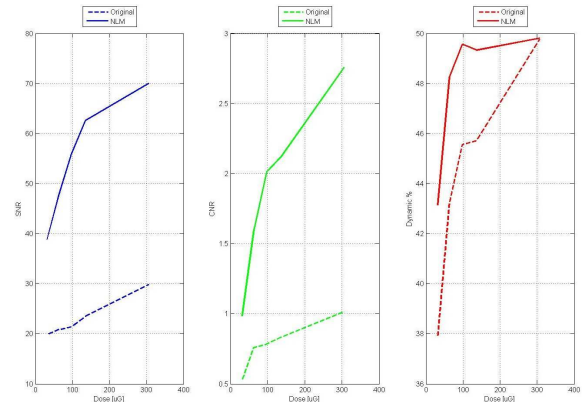
Fig. 4: Image quality metrics on the phantom image: left SNR, center CNR, right DYN. Dotted lines: no specific processing for the noise; continuous lines: proposed NL-means filter with adaptive parameters.
