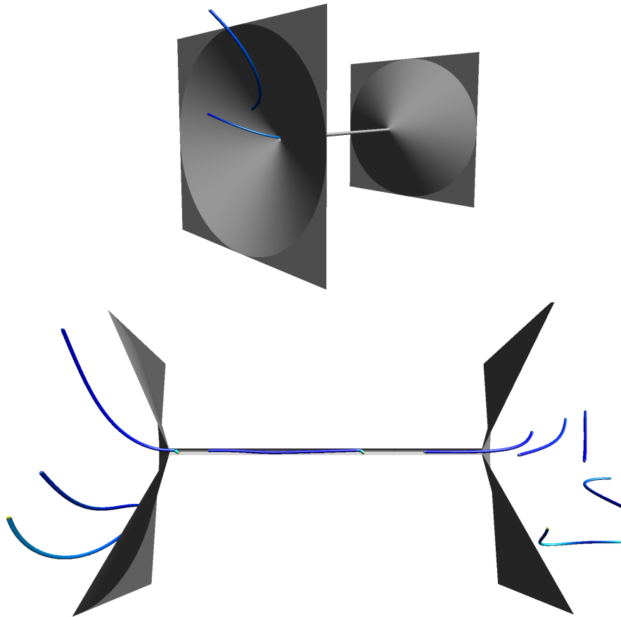
Figure 5: The double funnel case where the elastic rod must go through a very narrow passage (top) and a solution path (bottom) where the rod must go from the left side to the right side (view has been clipped for clarity).
