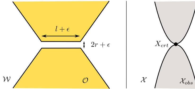
Figure 4: A critical narrow passage for an elastic rod represented in the workspace \mathcal{W} (left) and its equivalent illustrated in rod state space \mathcal{X} . As \epsilon tends to zero, the probability of sampling on X_{crt} also tends to zero.
