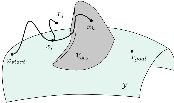
Figure 2: Illustration of the tree exploration in the state space \mathcal{X}_{adm} while sampling states on the submanifold of quasi-static contact-free states \mathcal{Y} . We can see that the resulting state of an extension step can lie on this submanifold as x_i , be in contact as x_k or be any state in \mathcal{X}_{adm} as x_j .
