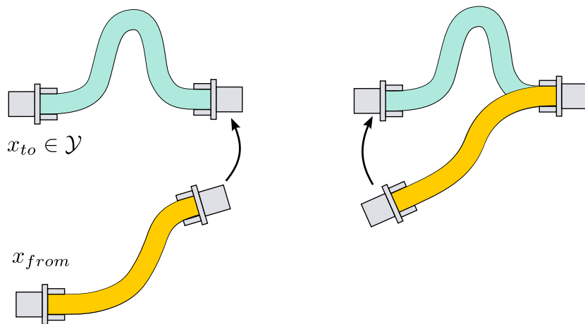
Figure 3: Illustration of the two steps approach for the local planner from a state x_{from} to a quasi-static state x_{to} . First, a randomly chosen gripper is manipulated to its respective goal (left). Once its goal is reached, the first gripper is fixed and the other one is manipulated the same way (right).
