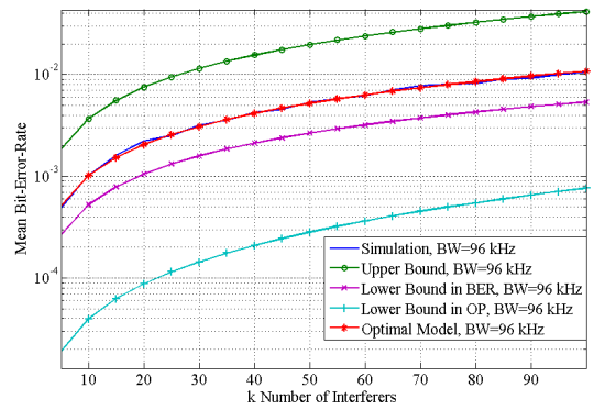
Figure 7. Mean BER as a function of k interferers, for BW = 96 kHz.
