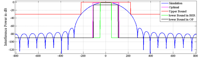
Figure 2. Behavior of the interference [dB] vs frequency difference \delta_f .
