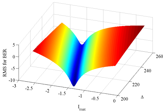
Figure 5. RMS for BER vs the couple (\Delta, I_{max}) , for I_{min} = -90 dB, k = 20 interferers and BW = 12 kHz.
