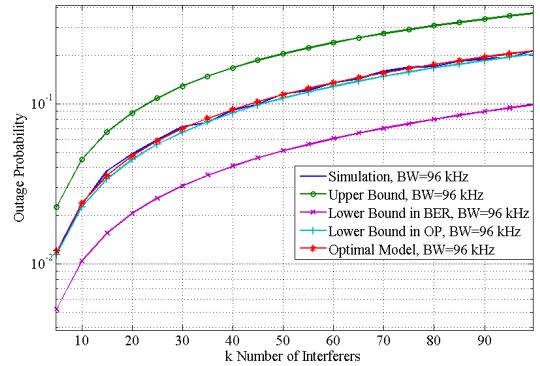
Figure 8. OP as a function of k interferers, for BW = 96 kHz.
