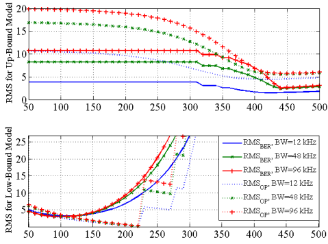
Figure 4. RMS for BER and OP vs \Delta , for k = 100 , different bandwidth lengths.
