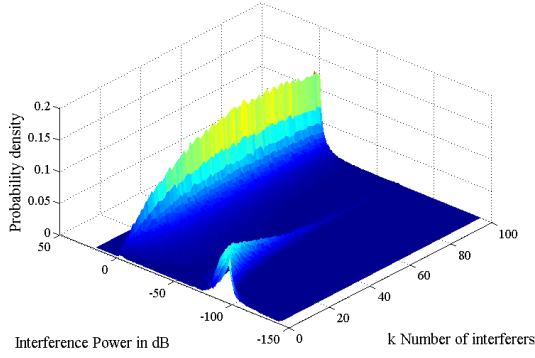
Figure 3. PDF of the aggregate interference power [dB], for k = 100 interferers, for BW = 12 kHz.
