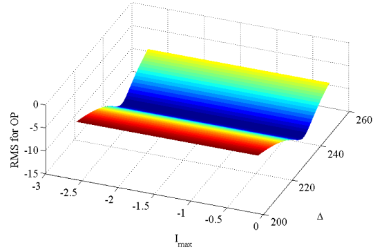
Figure 6. RMS for OP vs the couple (\Delta, I_{max}) , for I_{min} = -90 dB, k = 20 interferers and BW = 12 kHz.
