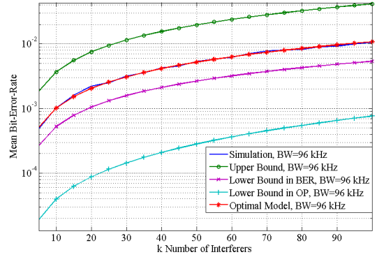
Figure 7. Mean BER as a function of k interferers, for BW = 96 kHz.
