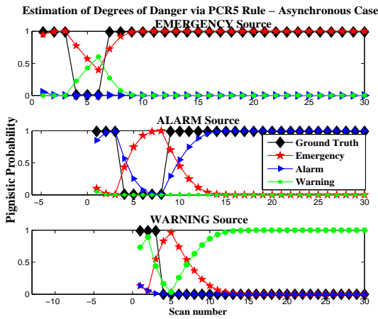
Figure 8: PCR5 rule Performance for danger level estimation.
