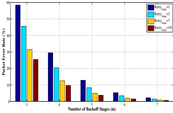
Fig. 11. Packet error rate for single band vs. number of backoff stages for various retransmission limits.
