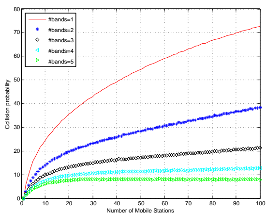
Fig. 3. Collision probability (%) vs. number of users with m=3 for various number of RTS bands.
