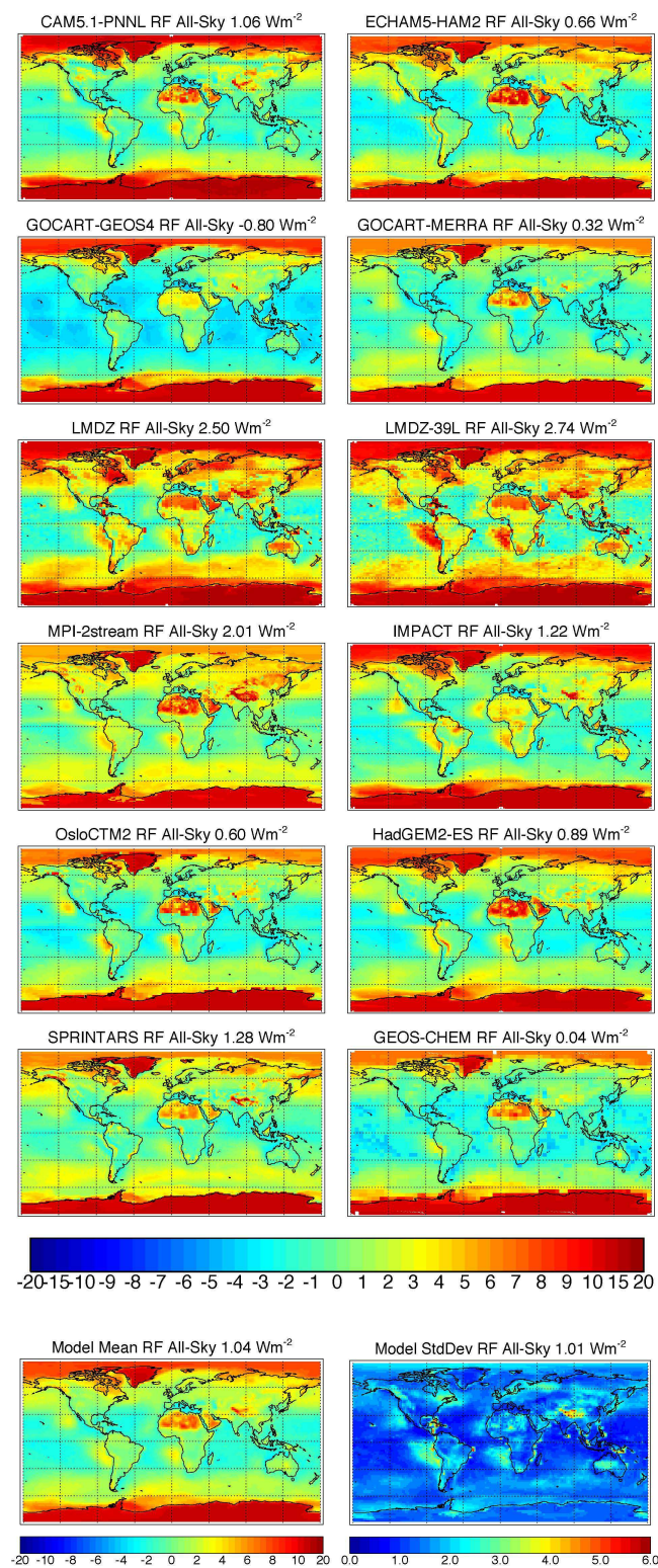
Fig. 9. Annual mean short-wave all-sky top-of-atmosphere radiative forcing between experiments with \text{AOD}=0.2 and \text{AOD}=0.0 distributed over the lowest two kilometers, holding \text{SSA}=0.8 and \text{ANG}=1.0 constant (FIX3-FIX0).
