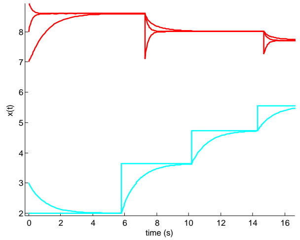
Fig. 1. Up: Consensus of the five agents grouped in 2 clusters. Down: Zoom in pointing out that the resets are not synchronized.
