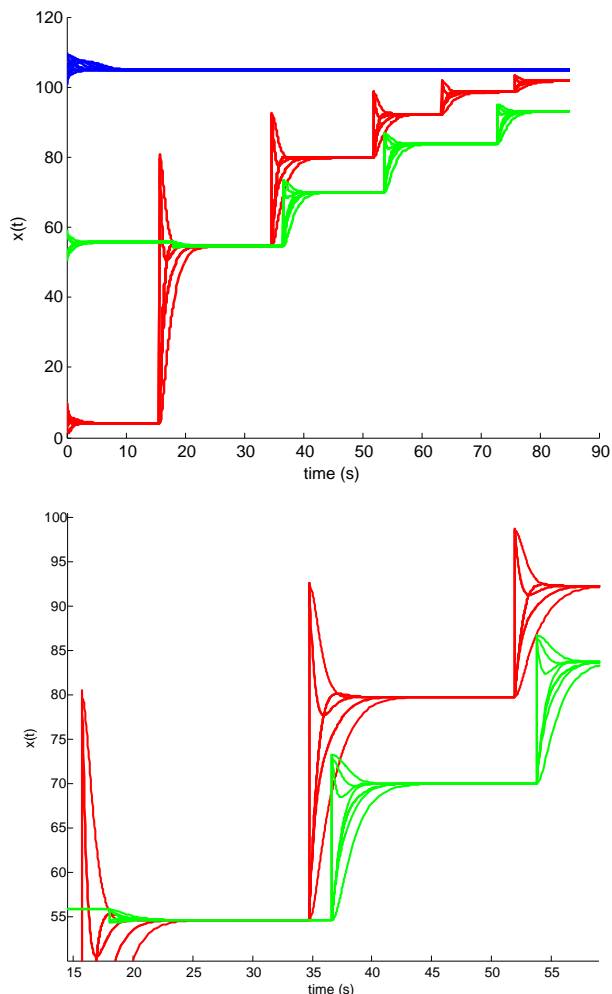
Fig. 2. Top : Trajectory of the reset system (2) with 30 agents grouped in 3 clusters. The overall interaction network topology among cluster is a tree. The top (blue) cluster influences the bottom (red) clusters which influences the middle (green) cluster. Bottom : zoom-in of the trajectory.
