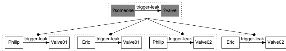
Fig. 3. Instantiation
