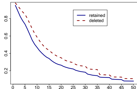
Figure 4: Badness scores of the links in the crawl analysis described in Section 4. The x axis shows the Badness scores of the documents which linked to the retained (“good”) and the deleted (“bad”) documents. The y axis shows the proportion of retained/deleted documents for which the Badness score is \geq x . (Lower Badness scores are better.)
