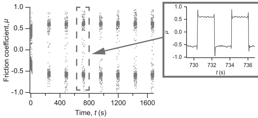
Fig. 6. Sequential measurement of the friction coefficient at F_N = 215.5 \text{ N} and v = 0.32 \text{ m s}^{-1} on d = 500 \text{ m} .
