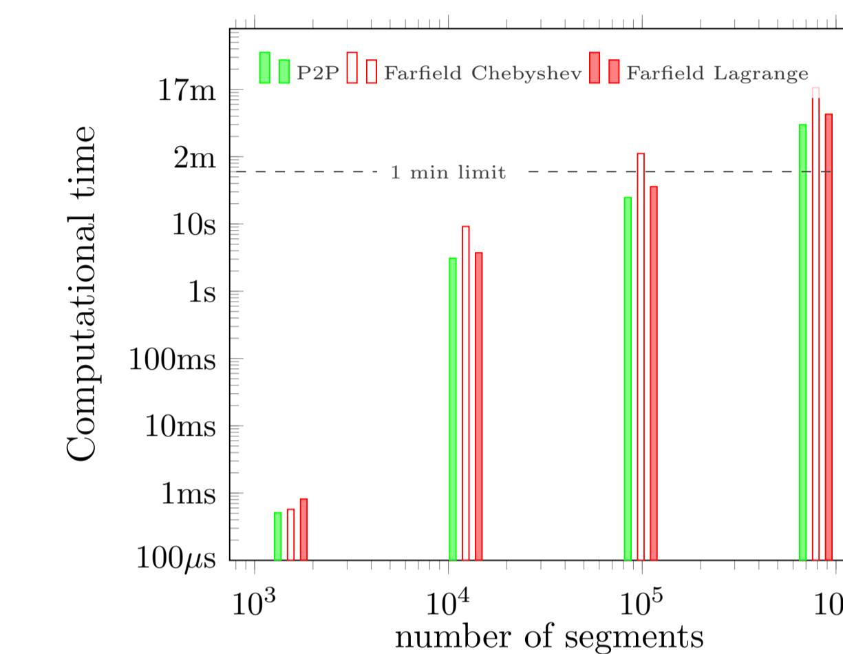
FIGURE 5: Isotropic near- and farfield computational time balancing for a uniform distribution of dislocation loops and increasing tree depth (left). An example of defects distribution and a propagating Frank-Read source (right).
