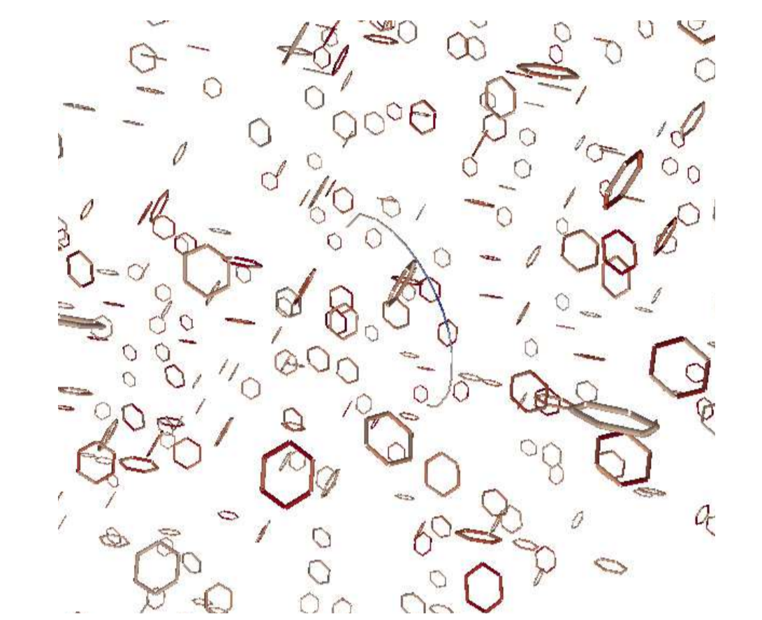
FIGURE 5: Isotropic near- and farfield computational time balancing for a uniform distribution of dislocation loops and increasing tree depth (left). An example of defects distribution and a propagating Frank-Read source (right).
