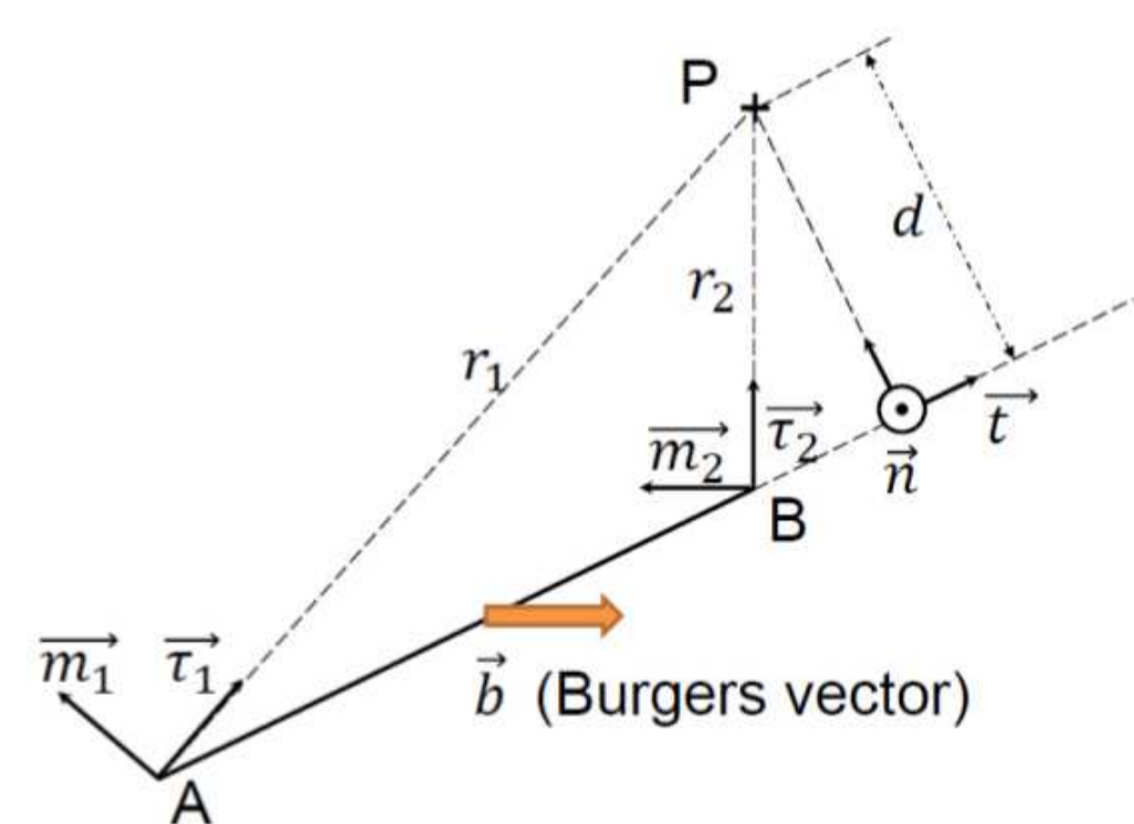
FIGURE 1: Notations for the stress created by segment AB on a field point P.
