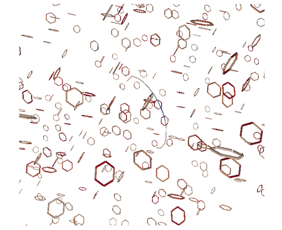
FIGURE 3: Near- and Farfield computational time balancing for a uniform distribution of dislocation loops and increasing tree depth (left). An example of defects distribution and a propagating Frank-Read source (right).
