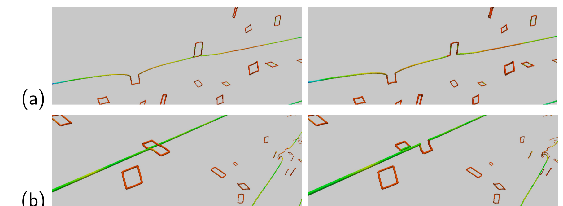
FIGURE 4: Evolution of 6 screw Frank-Read sources (top) inside a grain of Zr with a large density of defects ( d = 1.10^{22} \text{ m}^{-3} ). Elementary events (bottom): (a) double jog (b) dissociation.
