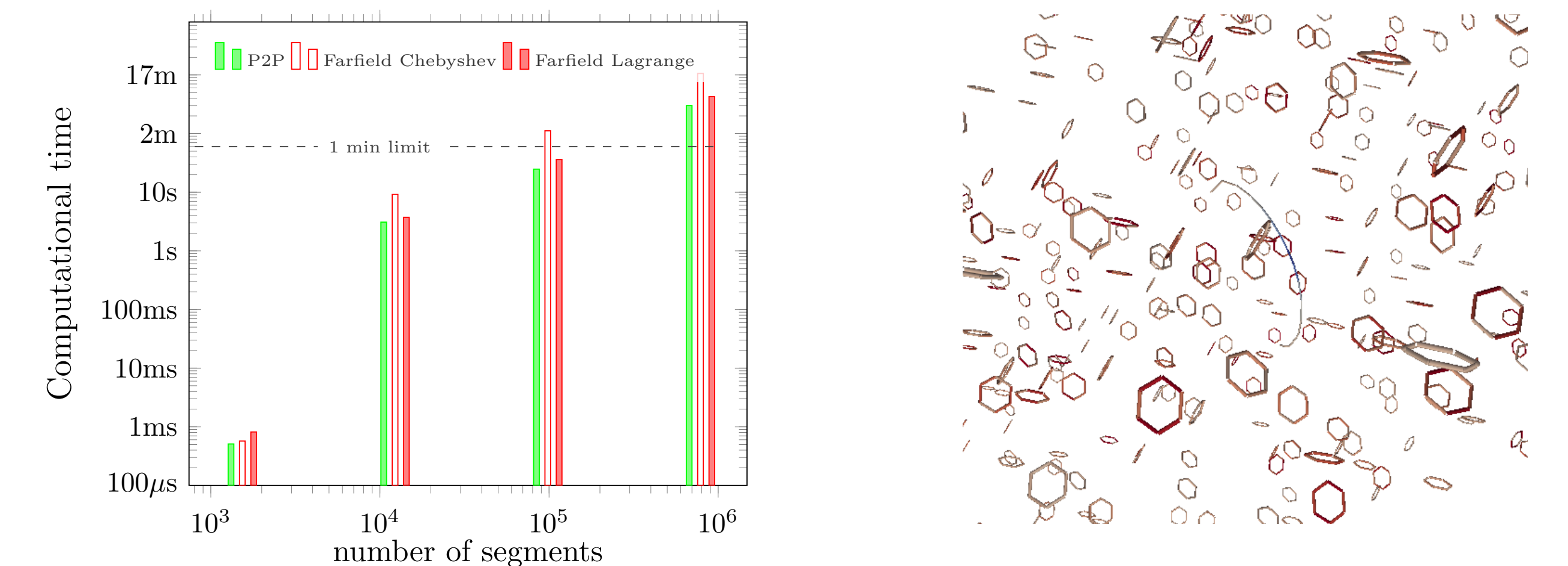
FIGURE 3: Near- and Farfield computational time balancing for a uniform distribution of dislocation loops and increasing tree depth (left). An example of defects distribution and a propagating Frank-Read source (right).
