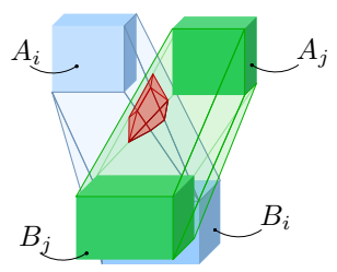
Fig. 5. Depiction of the sheath-sheath interference test; example of an intersection (in red) of the sheaths.
