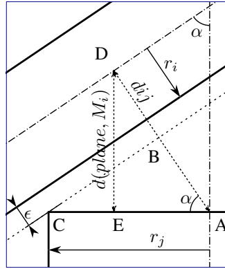
Fig. 10. Schematic of the "cap" situation in case one leg is right above - or below - the other, and parametrization.
