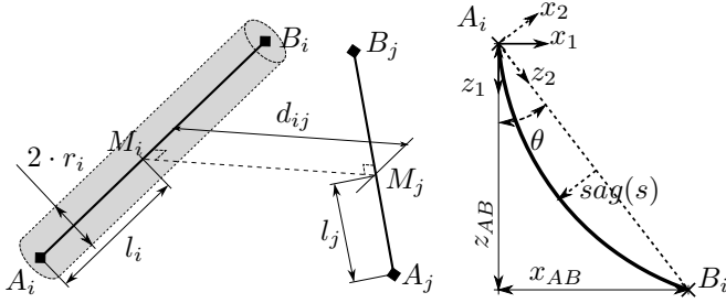
Fig. 6. Schematic of the two segments representing two legs of a parallel robot and parametrization for the minimum gap-based interference test.
