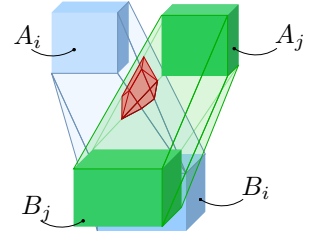
Fig. 5. Depiction of the sheath-sheath interference test; example of an intersection (in red) of the sheaths.
