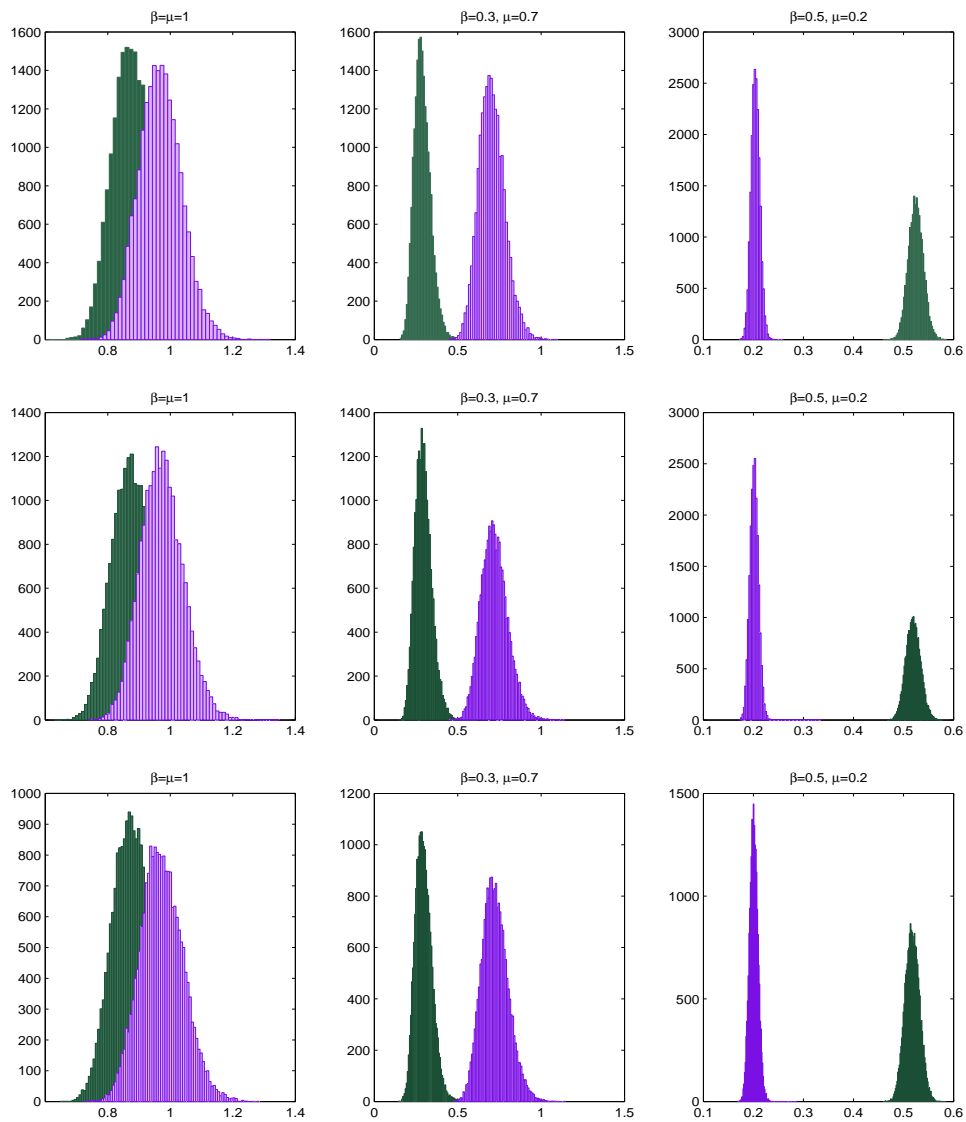
Figure 1: Frequency histograms based on 10000 for posterior densities estimate of \beta ( green ), and \mu ( violet ), for m = 5 , m = 10 and m = 15 with born-in of 20000 iterations in all cases. (For interpretation of the references to colour in the legend of this figure the reader is referred to the electronic version of this article).
