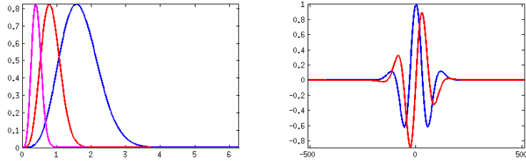
Figure 2: Analytic derivative of Gaussian wavelets ( k = 4 ). Left: Fourier transforms, with three different values of the scale parameter. Right: real part (blue) and imaginary part (red) of a wavelet in the time domain.
