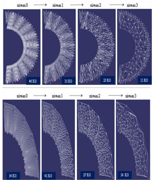
Figure 8 : example of two fragments simplification with maximum radius of curvature = 120^\circ .
