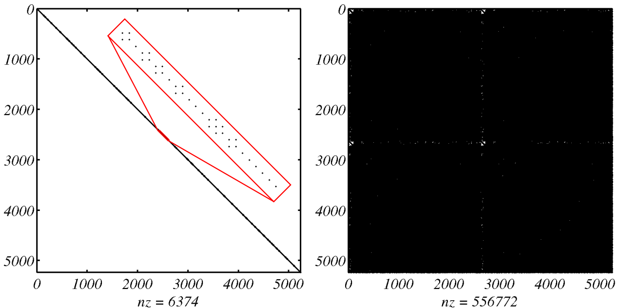
Figure 7: Non-zero elements of the quasi-diagonal preconditioner \mathbf{P}_{qd} (left) and comparison to those of the dual Schur complement \mathbf{S}^d (right).
