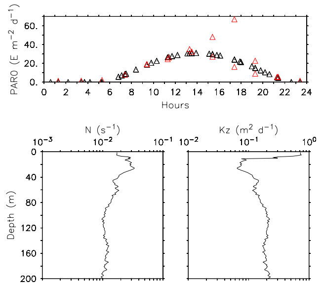
Fig. 2. Measured (14–15 August, 2009, red triangles) and fitted-from-data (black triangles) surface PAR (PAR0, upper panel), 4-day (14–16 August, 2009) averaged profile of measured Brunt-Väisälä frequency ( N , lower left panel) and derived profile of eddy diffusion coefficient ( K_z , lower right panel).
