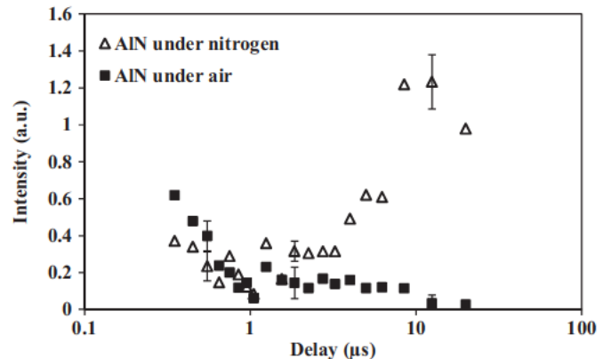
Fig. 4. Comparison between the temporal evolution of the AlN molecular band at 507.680 nm under nitrogen (triangle labels) and air (square labels) atmospheres.
