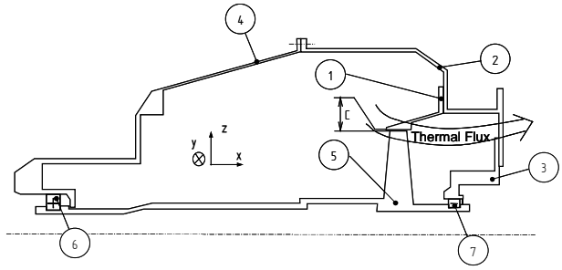
Figure 13: Simplified geometric model of a high-pressure turbine.
