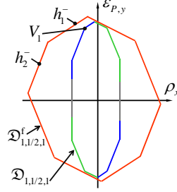
Fig. 16. Inclusion of the calculated polytope \mathfrak{D}_{1,1/2,1} in the functional polytope \mathfrak{D}_{1,1/2,1}^f
